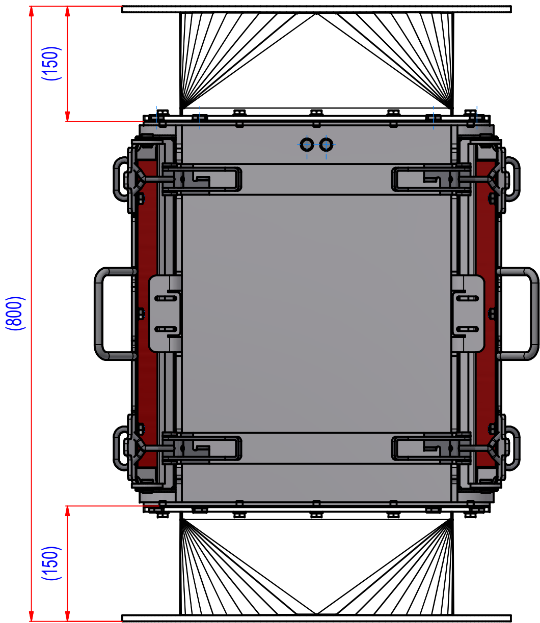
OPTION: SBPN353500 WITH ADAPTER TO DN350
