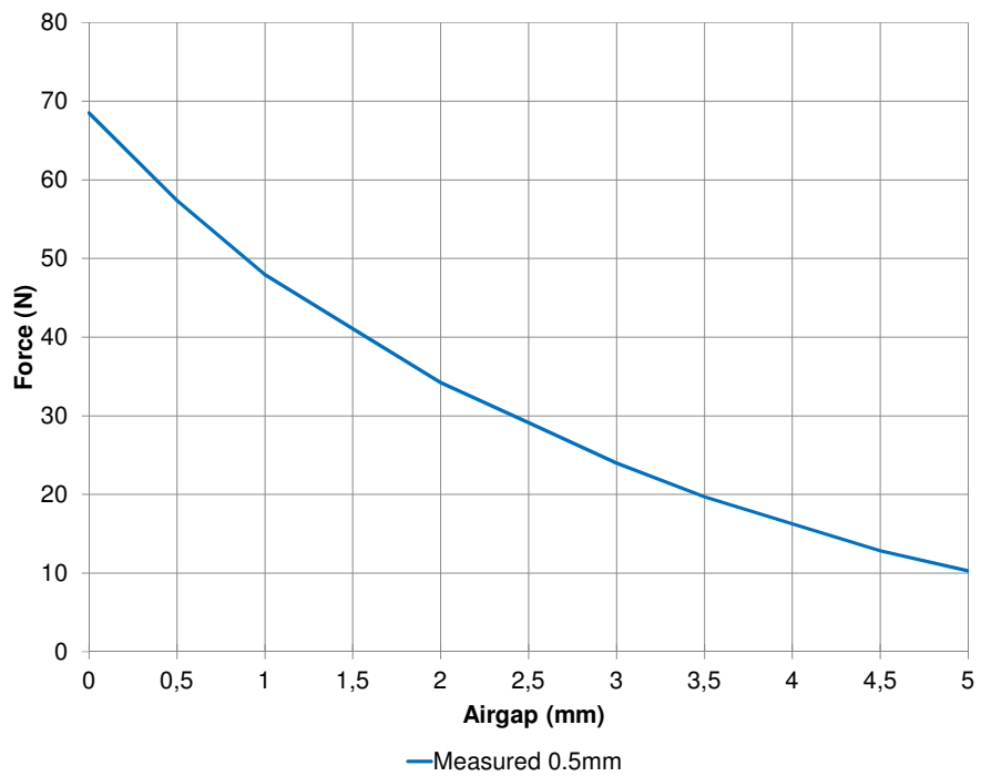
TPGC040088 Holding force curve plate thickness 0,5mm
