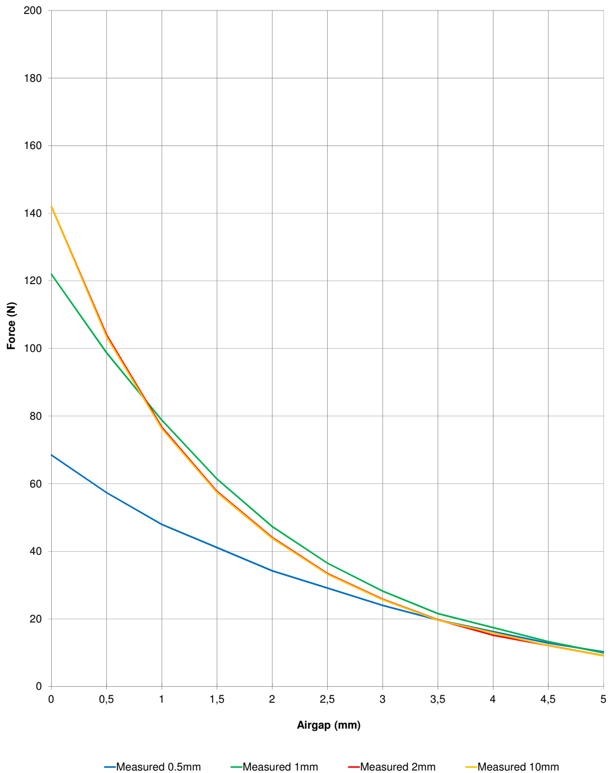
TPGC040088 Holding force curve plate thickness 0,5-10mm
