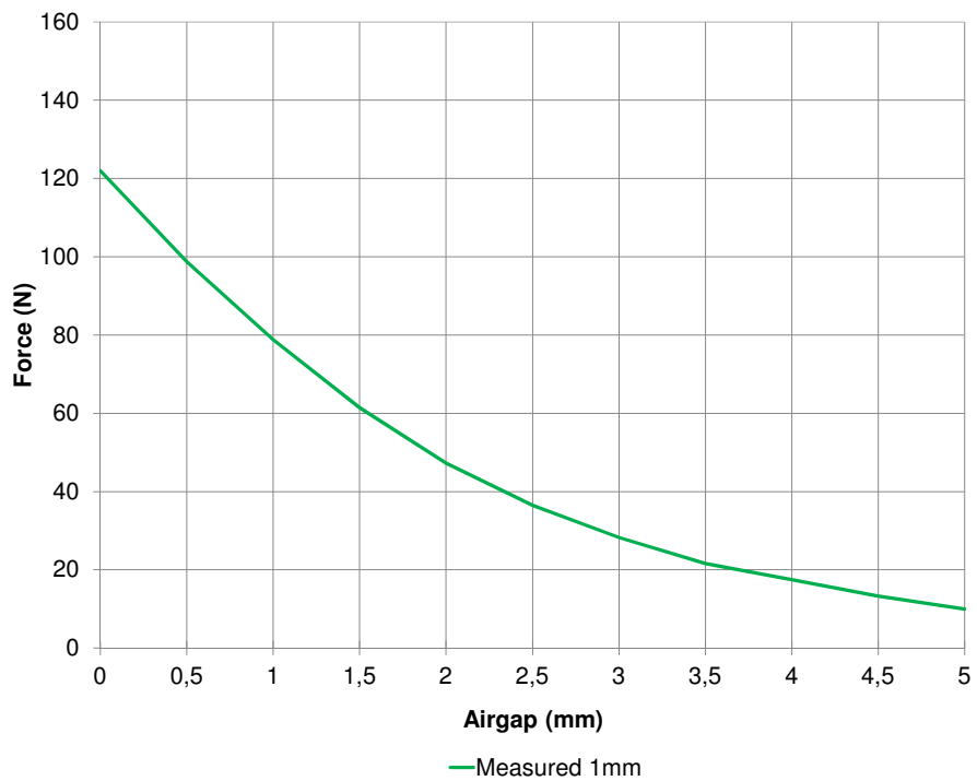
TPGC040088 Holding force curve plate thickness 1mm
